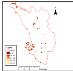
Figure 9: Water bodies map
