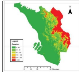
Figure 3: Elevation map
