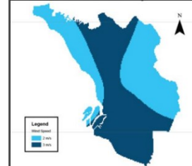
Figure 5: Wind contour map
