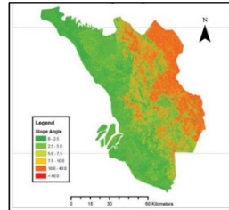
Figure 4: Slope map
