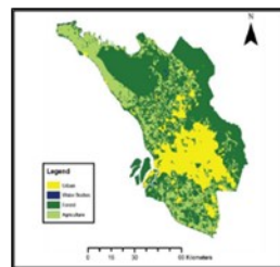
Figure 6: MODIS land map
