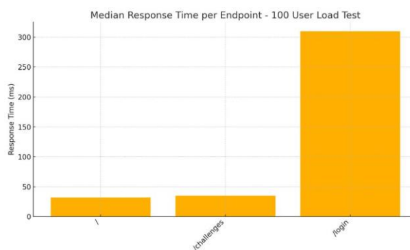
Fig. 3 Locust Results with heavy load testing (100 users)
