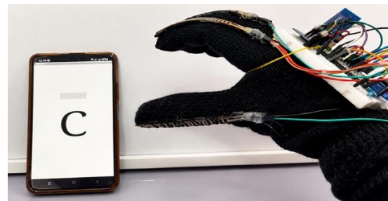
Fig. 3. ASL "C" output in display [3]
