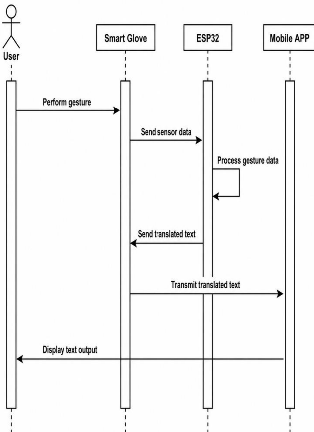
Fig. 8. Sequence Diagram
