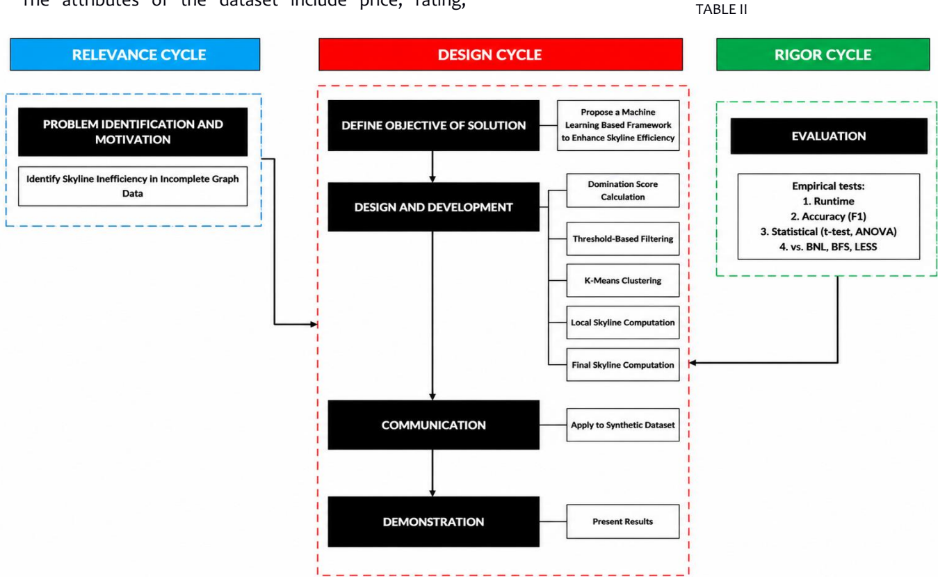
Fig.2. Proposed Methodology based on DSRM
