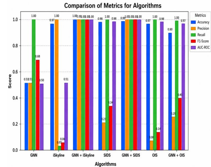
Fig 7. Comparison of Algorithms
