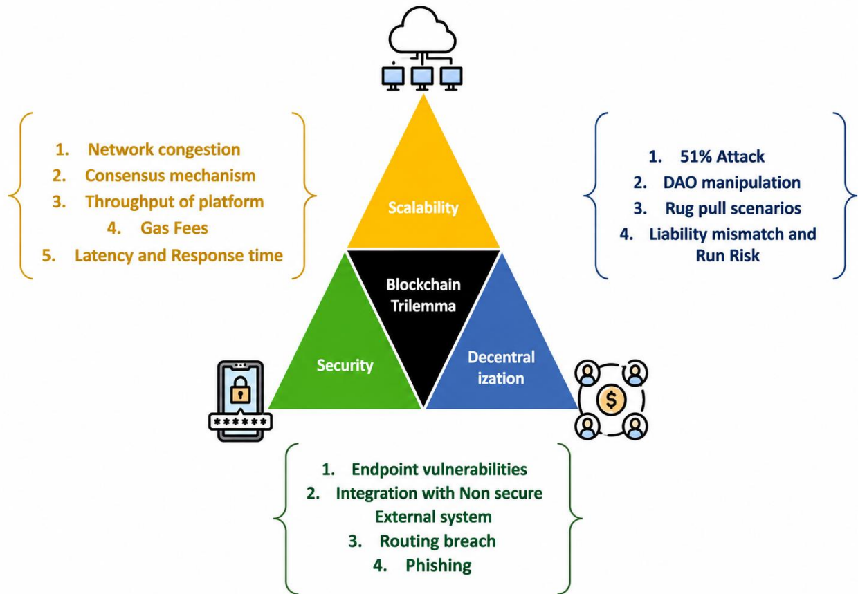
Fig 1: Blockchain Trilemma
