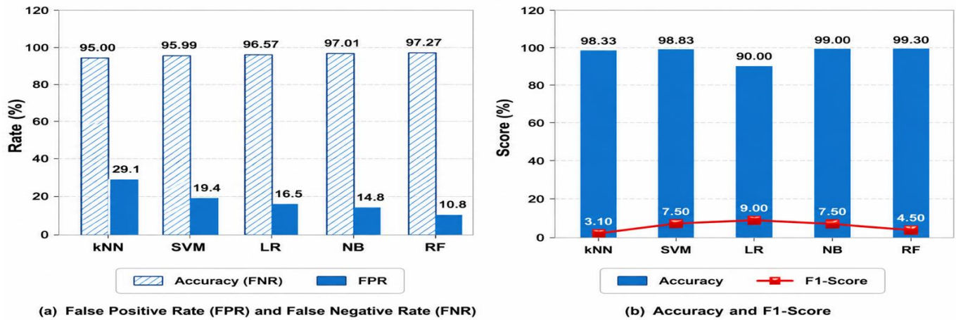
Fig. 3 3-gram scareware detection (left) and netflow scareware detection (right)
