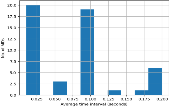
Fig. 3 Distribution of AIDs by average time interval, excluding AIDs with average time intervals greater than 0.25 second AID to decrease. Overall, a faithful CAN bus model should not only incorporate the dynamics of frame timing under normal operation, but also during different attack scenarios,
