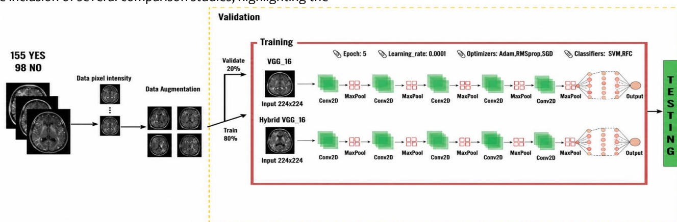
Fig. 1 The Training Model
