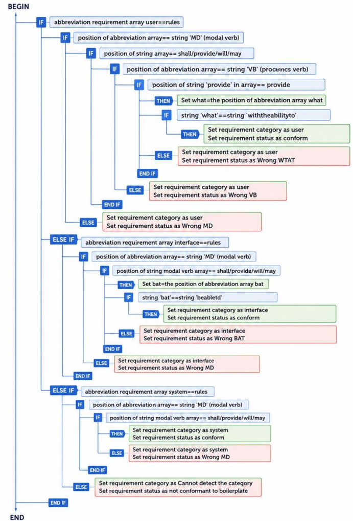
Fig. 5 Algorithm for Matching Requirements
