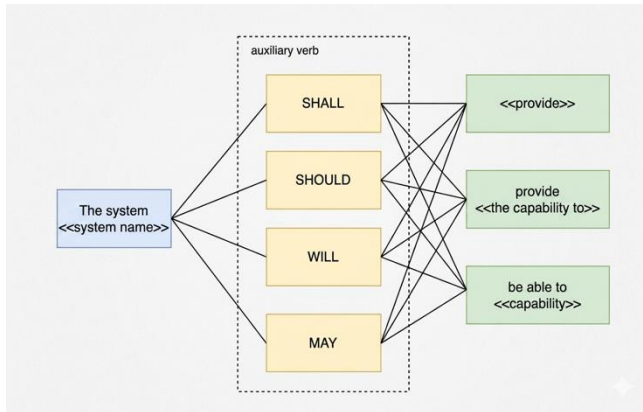
Fig. 1 Core requirement for IREB Boilerplate [2]
