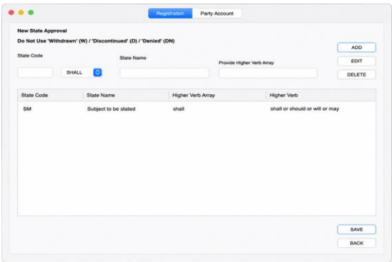
Fig. 8 Adding Requirements
