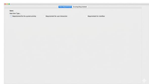
Fig. 6 Boilerplates Option
