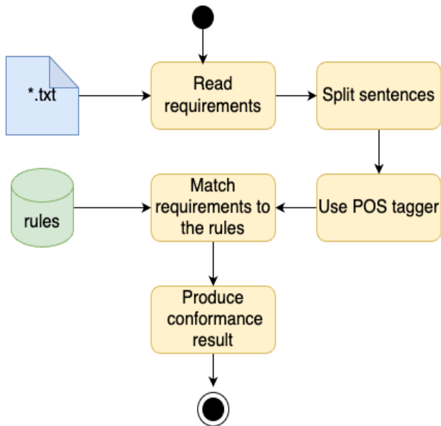
Fig. 4 Process in RCT
