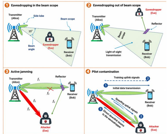
Fig. 6 Illustration of the methods to mitigate eavesdropping/jamming threats for 6G physical layer.
