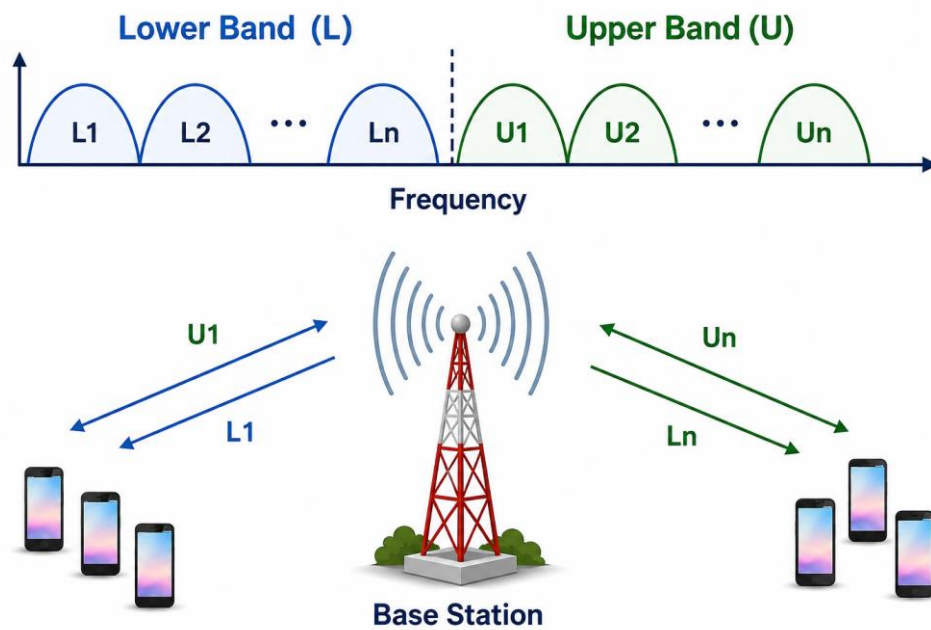
Fig. 2 The 2G cellular TDMA communication system[23]
