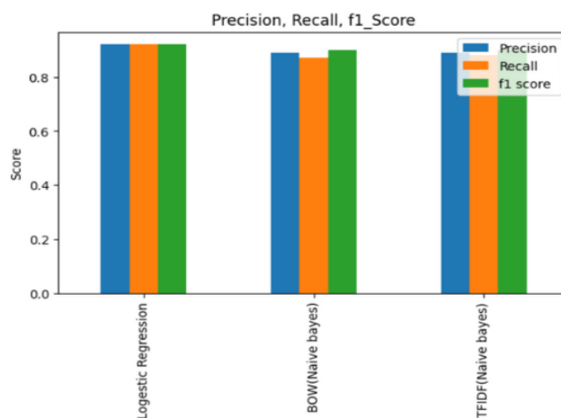
Fig. 10 Precision, Recall and F1-Score comparison
