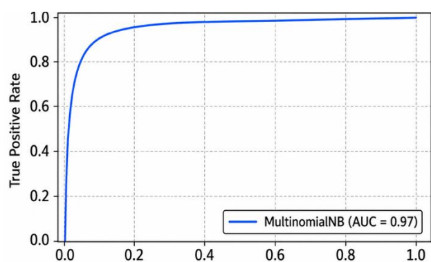
Fig. 9 ROC Curve for Naive Bayes with TF-IDF
