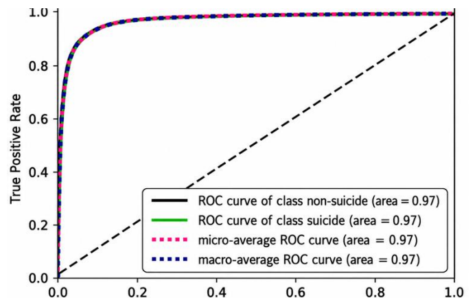
Fig. 7 ROC Curve for Logistic Regression model with Doc2vec
