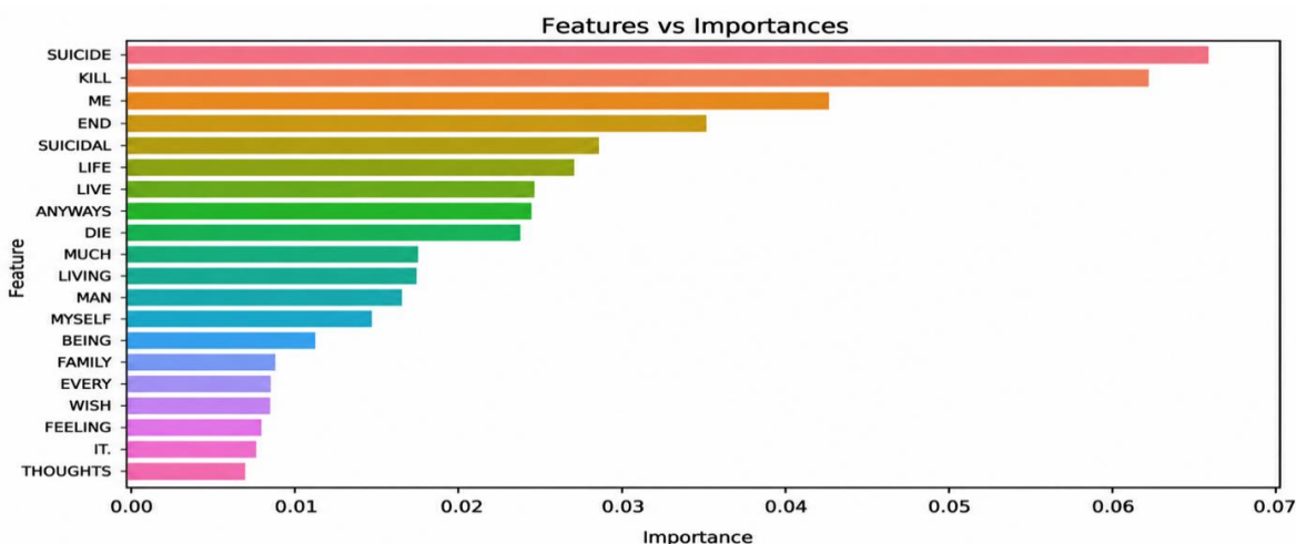
Fig. 11 Suicidal feature importance
