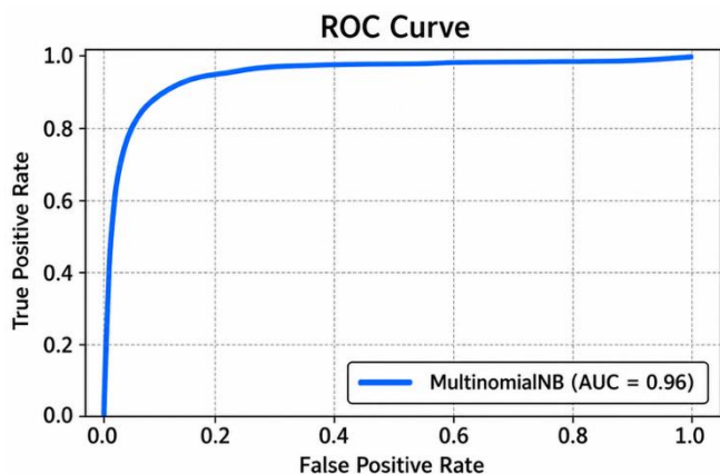
Fig. 8 ROC Curve for Naive Bayes with BOW
