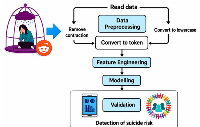
Fig. 1 Methodology Flowchart
