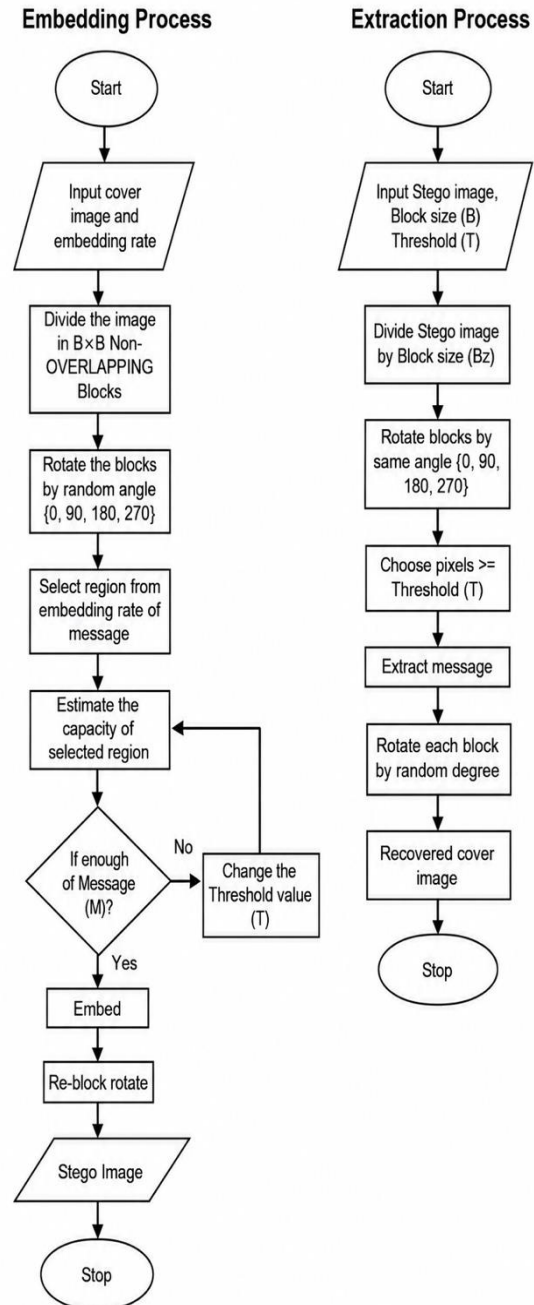
Fig. 5 Flowchart of EBE method
