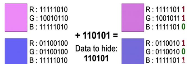
Fig. 3 Least significant bit of a 8-bit binary array
