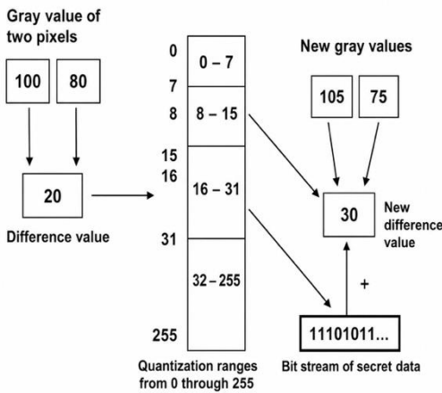
Fig. 4 Data embedding process of Wu-Tsai's PVD method
