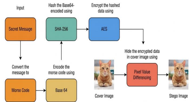
Fig. 7 Flow Diagram of the Proposed Framework
