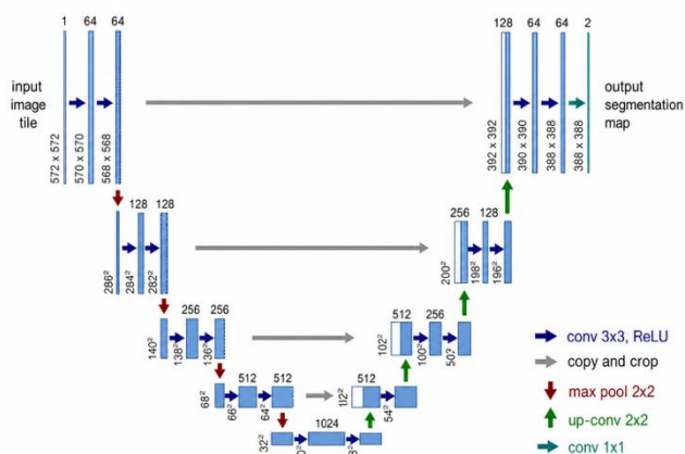
Fig. 2 Architecture of U-Net
