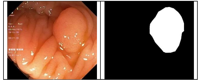
Fig. 5 Sample Dataset
