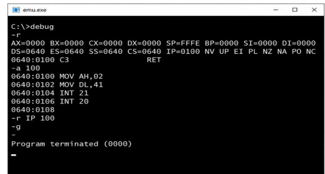
Fig. 1 Running debug.com on vDOS
