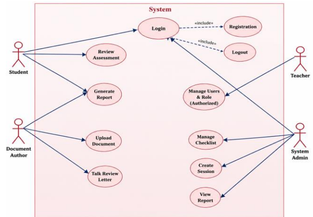
Fig. 2 Use case diagram for e-Review
