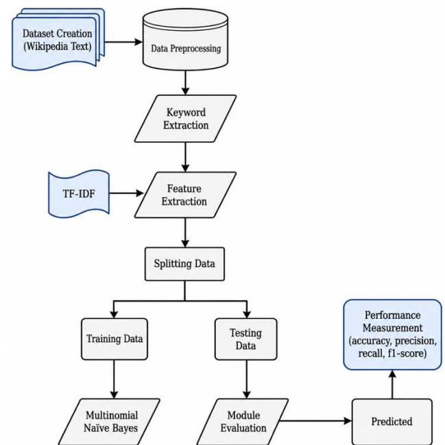
Fig. 1 Webpages Classification Flowchart
