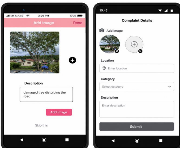
Fig. 4 (a) Add image page (b) Complaint details page
