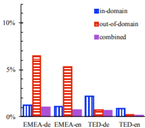
b) Out-of-Vocabulary (OOV) rates by tokens
