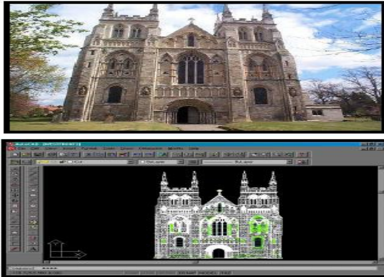
Figure 7: Selby Abbey, Selby West Yorkshire: (top) Photographic image (below) Photogrammetric output in CAD format prepared by the Downland Partnership Ltd. (Courtesy: Field Archaeology Specialist Ltd.)
