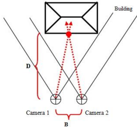
Figure 1: The principle of close-range photogrammetry for photographing a building in order to provide a stereo-pair photograph.
