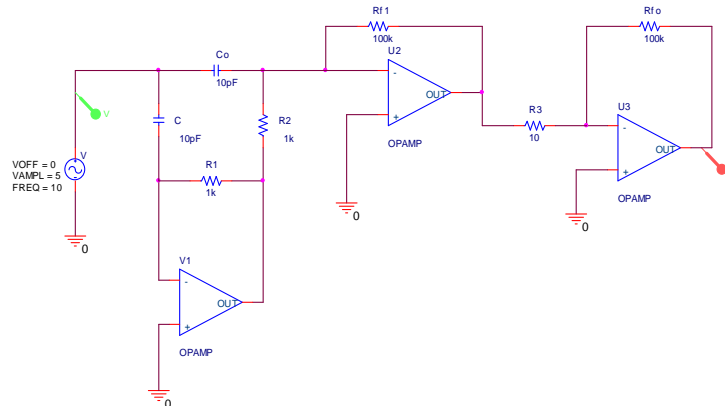
Fig. 4(a): Simulation Circuit for balanced condition.
