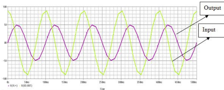
Fig. 5: PSPice simulation result for unbalanced condition (with C_x=30\text{pF} ).
