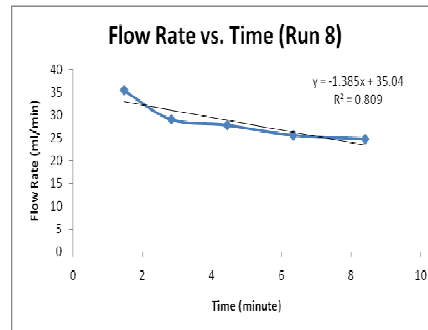
Fig. 4: Graphs for flow rate vs. time under room temperature. The microfiltration was operated at 28 °C; TMP, 4.5 psi and viscosity of sample used was 2.39 cP. An identical pattern of flow rate was observed with runs 1, 3 and 4.
