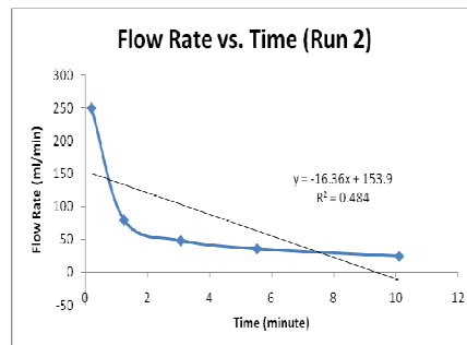
Figure 3: Graphs for flow rate vs. time under cold temperature. The microfiltration was operated at 4 °C; TMP, 4.5 psi and viscosity of sample used was 2.13 cP. An identical pattern of flow rate was observed with runs 1, 3 and 4.
