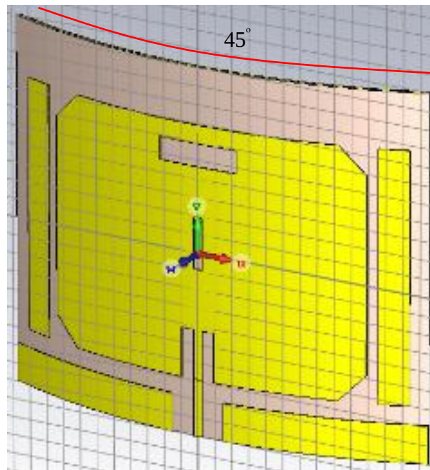
Figure 8. Antenna on 45^\circ bend curvature in CST.
