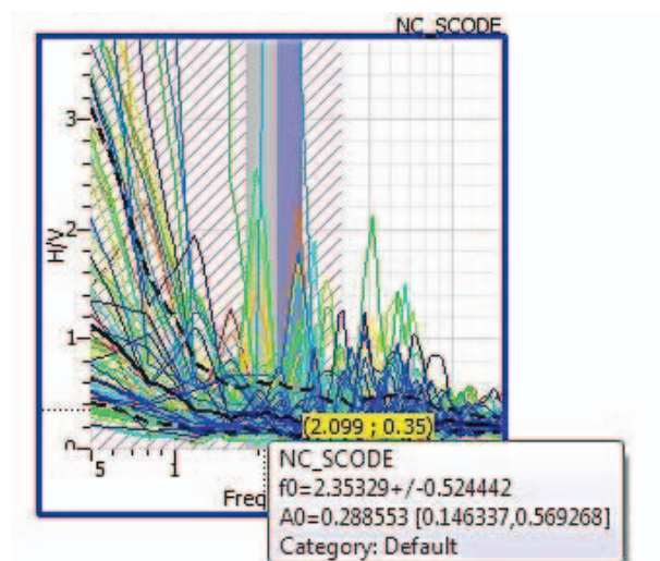
Fig. 9: The display of H/V graph at Majapahit Street with the results of natural frequency ( f_0 ) 2,35329 and amplification ( A_0 ) 0,288553.
