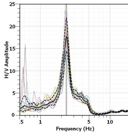
Fig. 3: The H/V amplitude versus frequency curve was obtained by using HVSR analysis [14].
