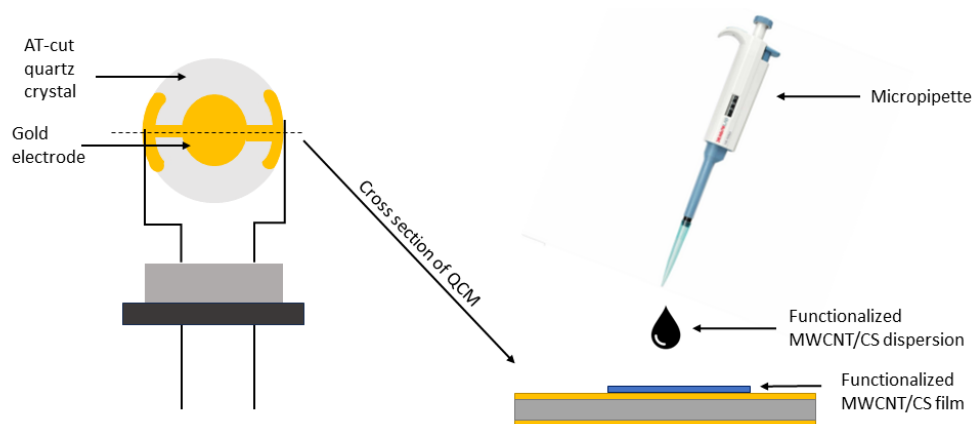
Fig. 2. Schematic illustration of the drop-casting process for depositing the MWCNT–COOH/CS composite sensing layer onto the quartz crystal microbalance (QCM) surface.
