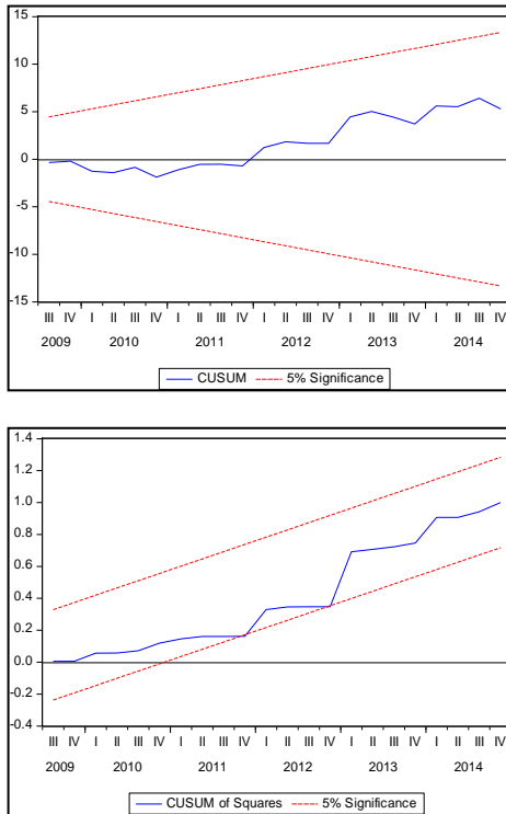
FIGURE 3 CUSUM and CUSUMSQ Tests for Housing Affordability (Conventional Home Loan)
